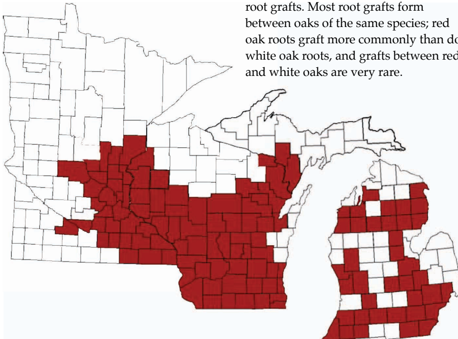
Figure 1. This map shows the county distribution of oak wilt in Michigan, Minnesota and Wisconsin in 2010. Map produced by the USDA Forest Service, Northeastern Area–Forest Health Monitoring GIS Group.
